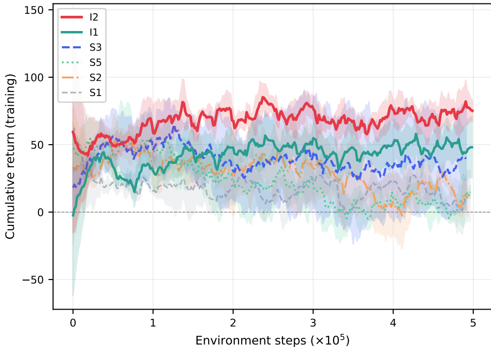
Training return (EWMA-50, mean \pm std)
